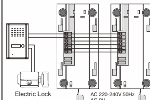
RL-3208DD WIRING DIAGRAM
