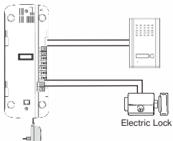
RL-3207A RL-3208A WIRING DIAGRAM
