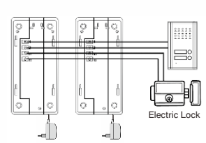
RL-3207AA RL-3208AA WIRING DIAGRAM
