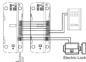
RL-3207CC WIRING DIAGRAM
